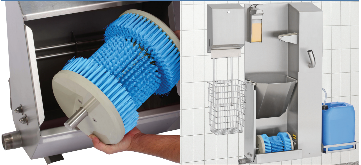
Hygienestation Solo Traditio Complete Typ 23822
