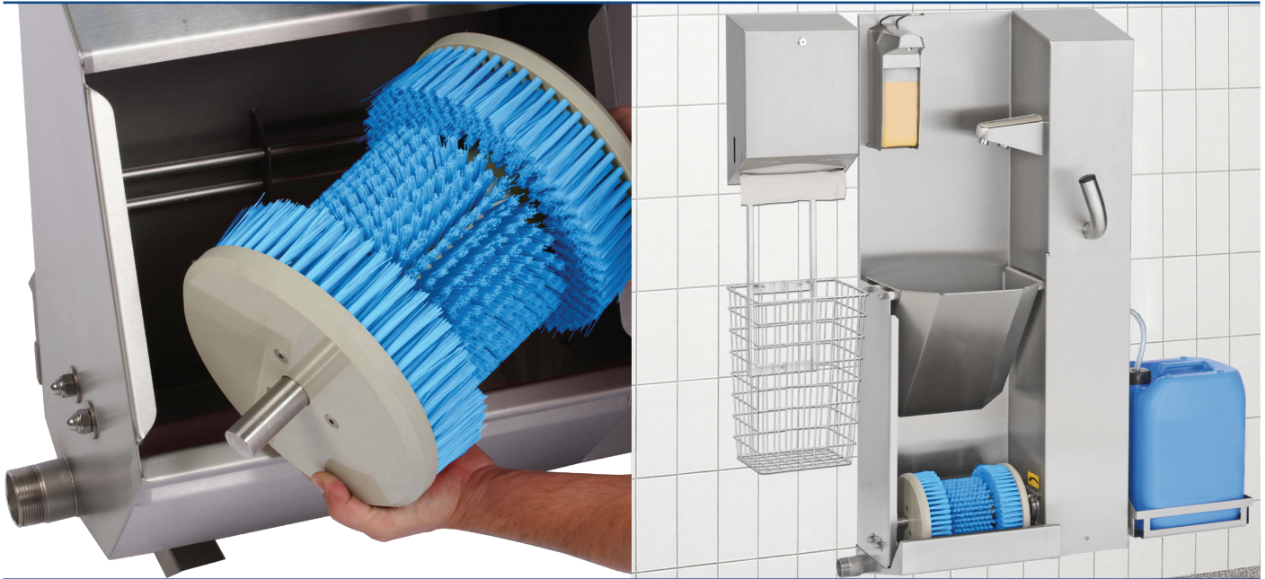
Hygiene Station Solo Traditio Complete Type 23822
