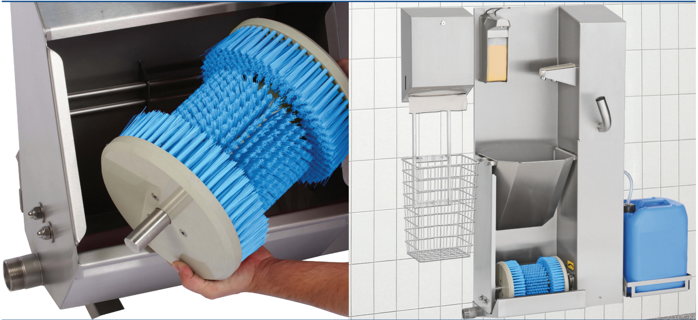
Hygiene Station Solo Traditio Complete Type 23822
