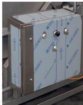
Optional: Control cabinet on the side with control and hydraulics
