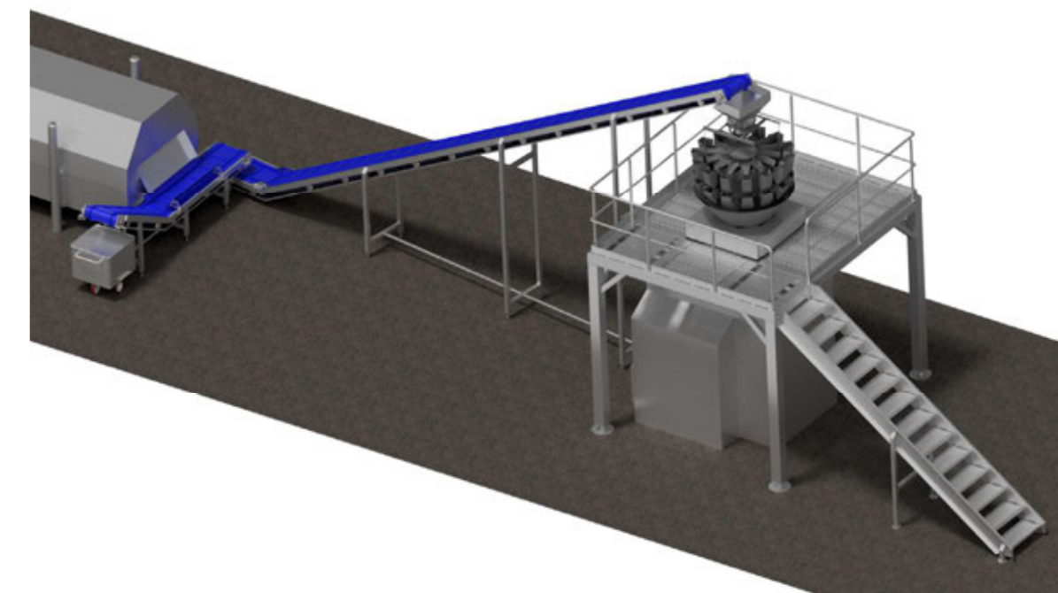
Image 43 Conveyor with platform
