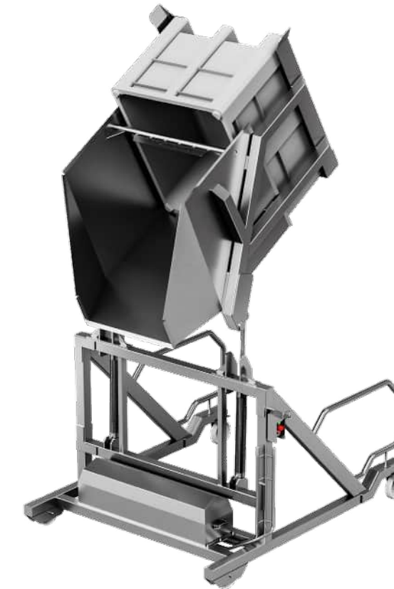
Bild.40 Swingloader-1000
